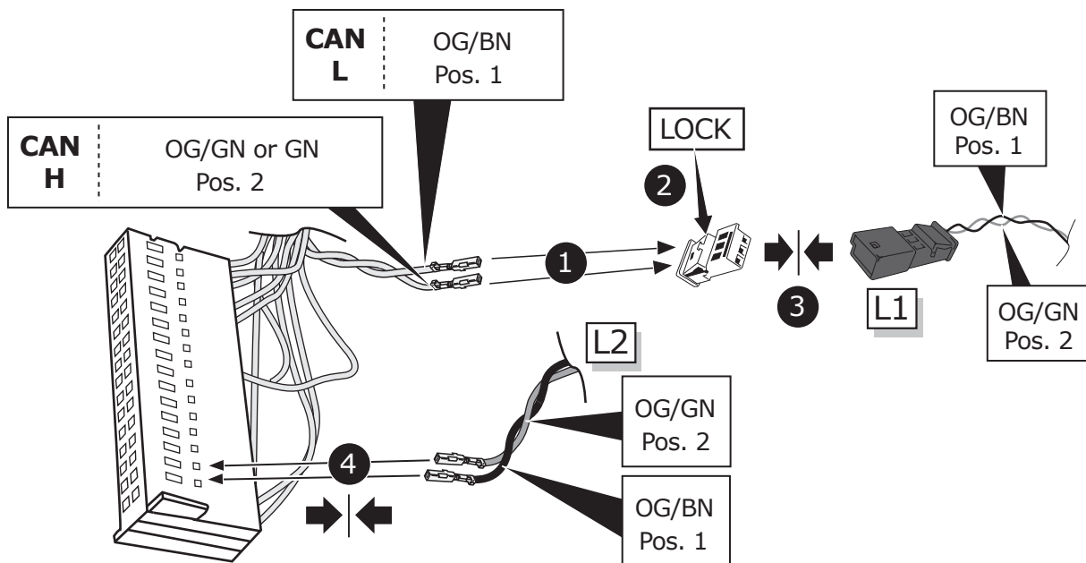
BU Connector 32 pole
