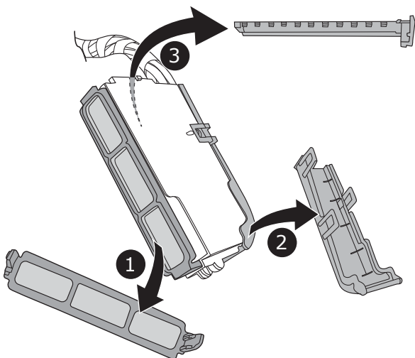
Fusebox 5 RD
